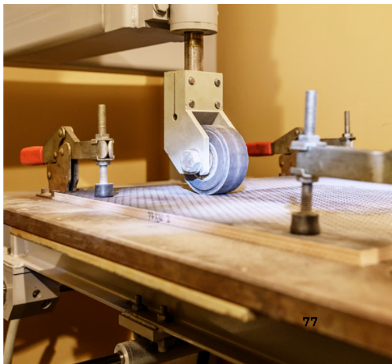
Figure 3.4. Determination of the effect of loaded heavy duty castors
