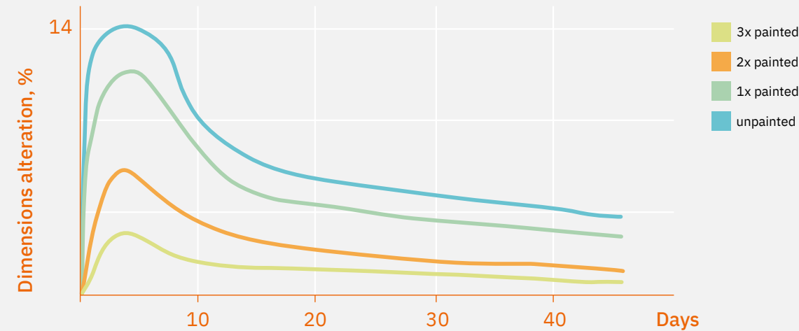
Figure 5.7. Dimension alteration of 18 mm plywood panel overlaid with phenol film, in %, 2 cm from the edge, after immersion in water for 48 h and drying
