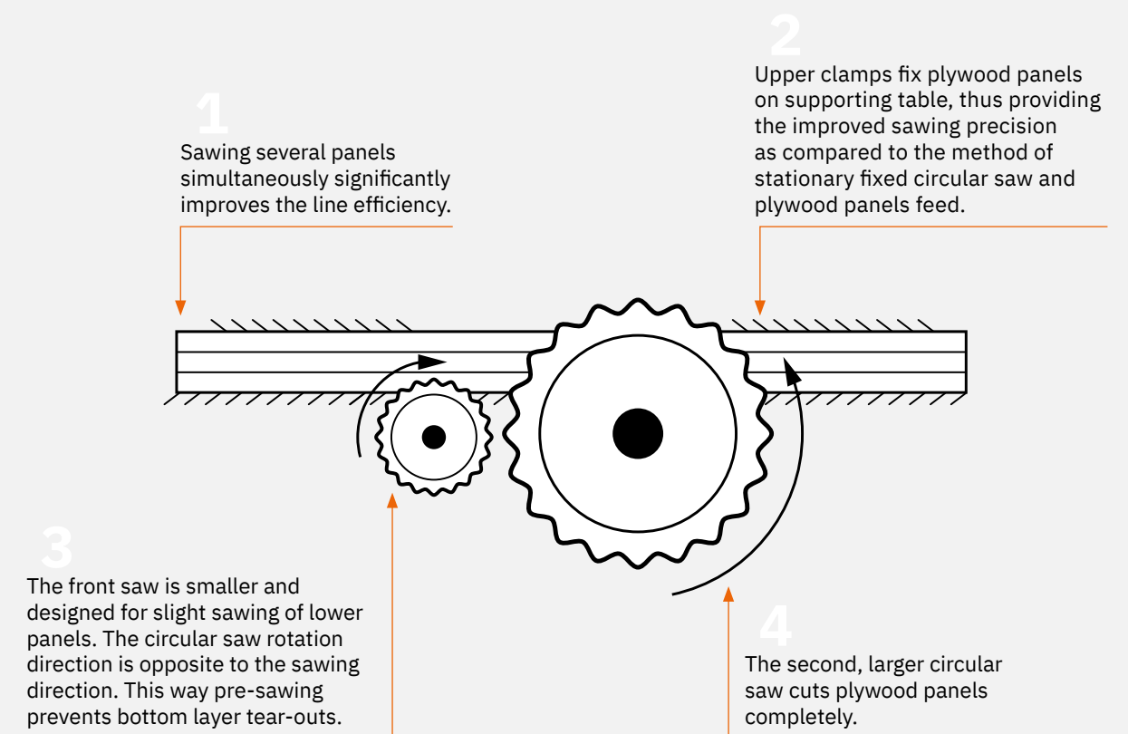
Figure 2.3. Plywood cutting scheme
