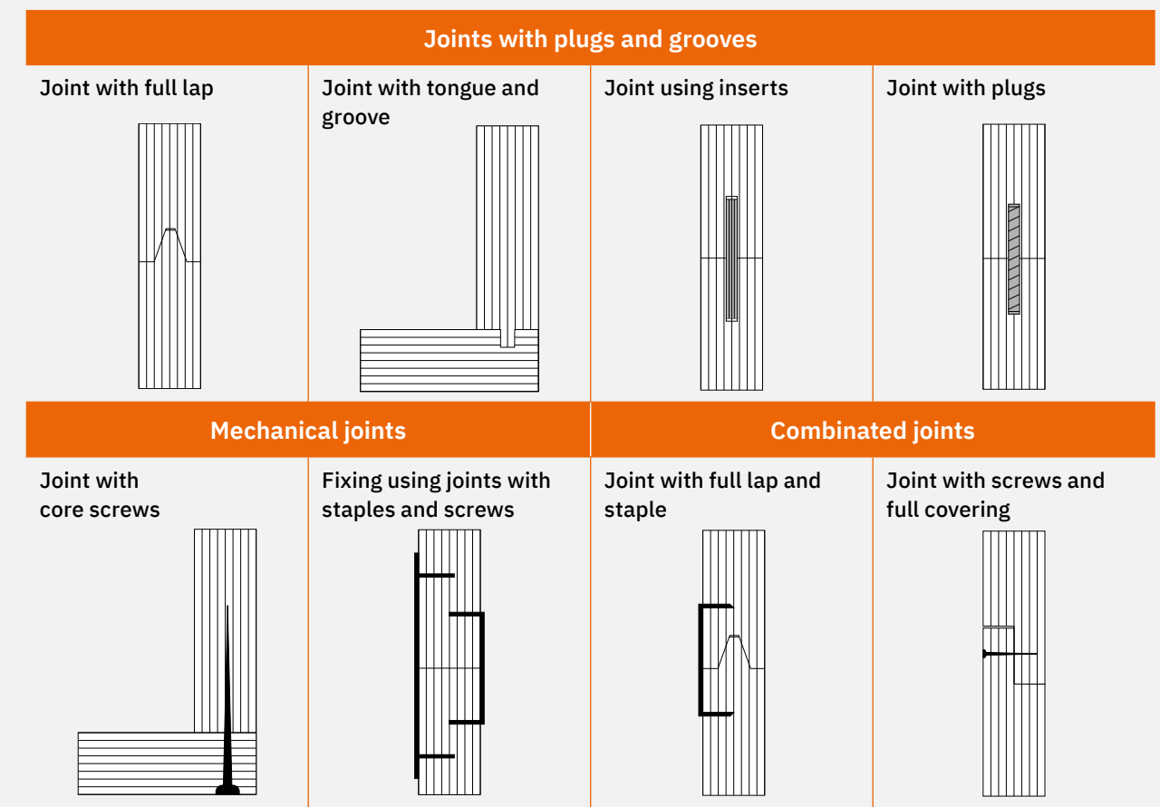
Figure 5.6. Joint types
